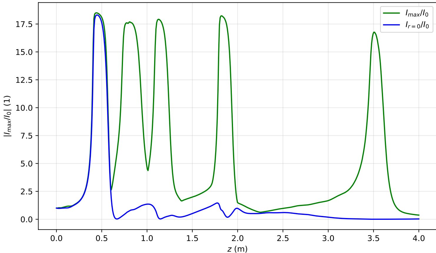
I_{max}(x = 0, y = 0, z)/I_0 , Pin=6.0Pcr, noisy input, artificial time
